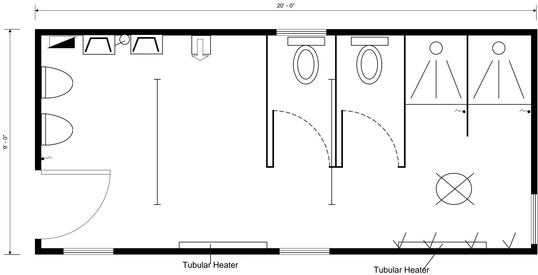
Stock 20' x 9' Toilet Shower unit. Timber Textured
